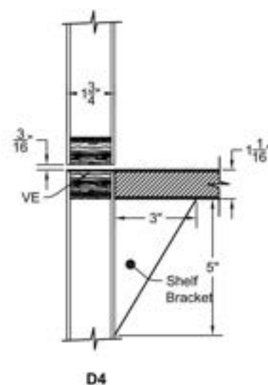
SHELF APPLIED TO DOOR FACE
